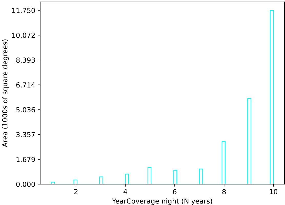
roll_pause_mjdp365_v3.4_10yrs u band: YearCoverage night
