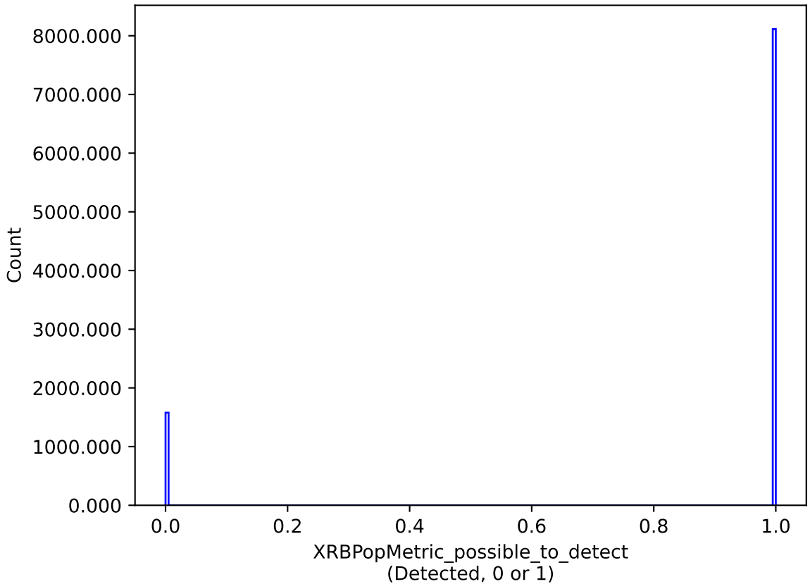
roll_pause_mjdp365_v3.4_10yrs : XRBPoMetric_possible_to_detect
