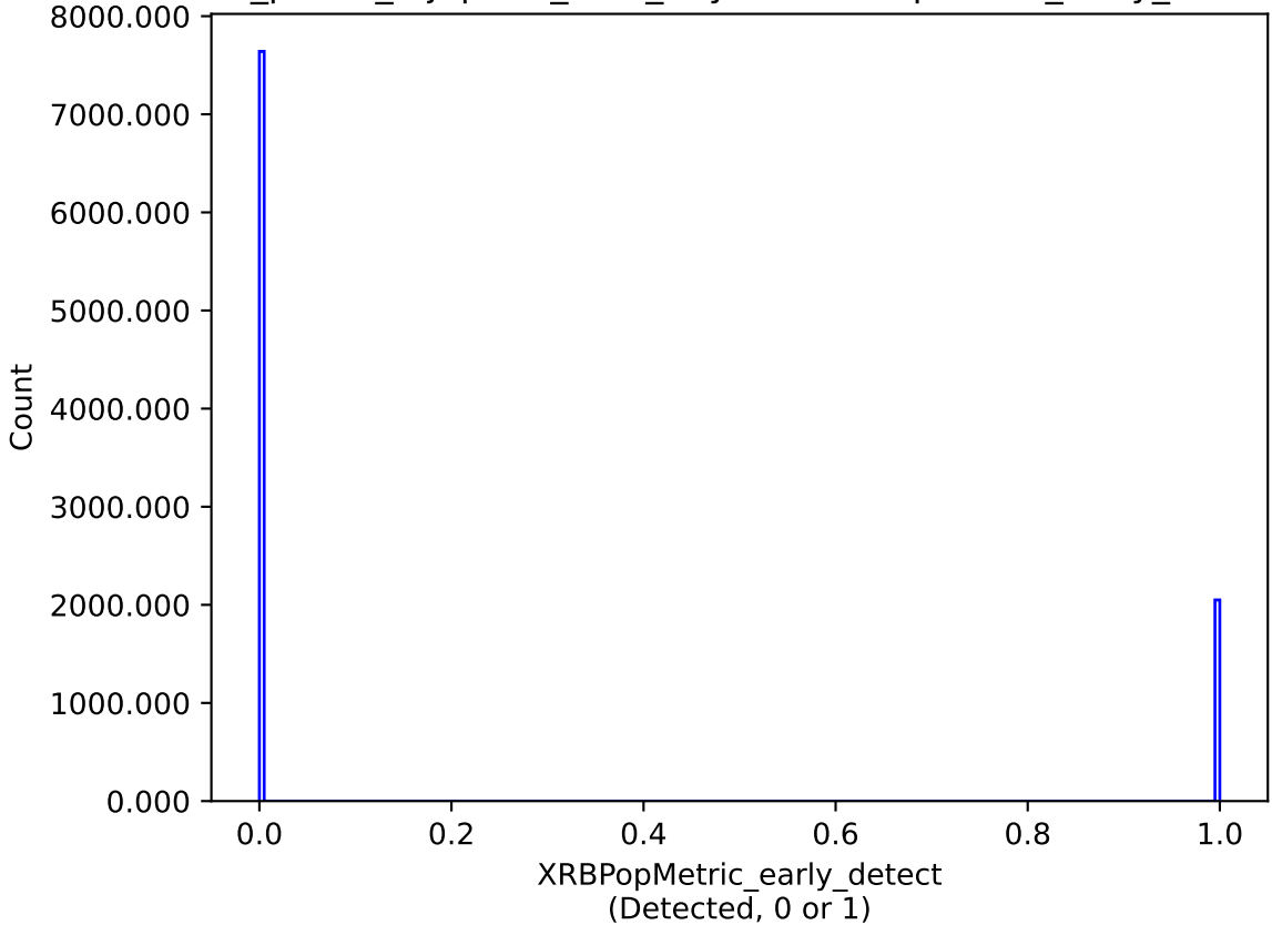
roll_pause_mjdp365_v3.4_10yrs : XRBPopMetric_early_detect
