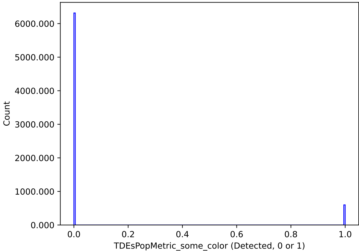
roll_pause_mjdp365_v3.4_10yrs : TDEsPopMetric_some_color
