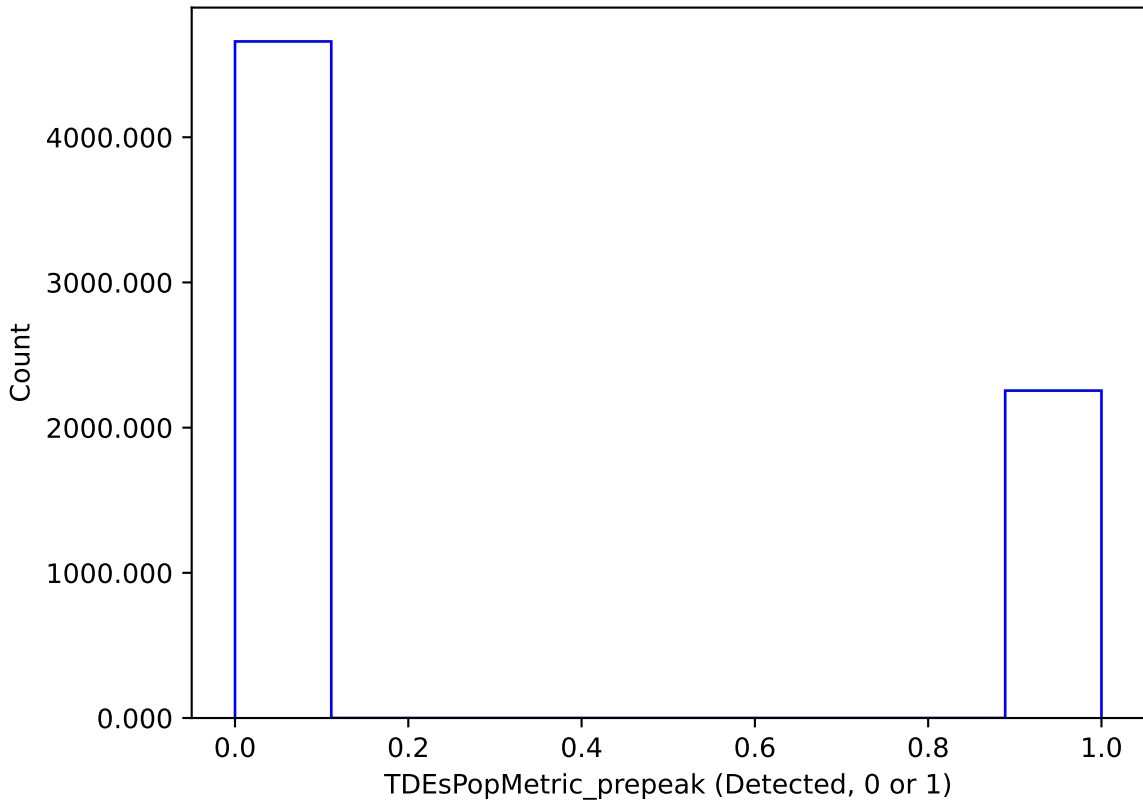
roll_pause_mjdp365_v3.4_10yrs : TDEsPopMetric_prepeak
