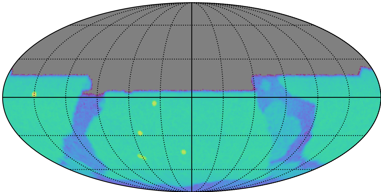
roll_pause_mjdp365_v3.4_10yrs u: SurfaceBrightLimit
