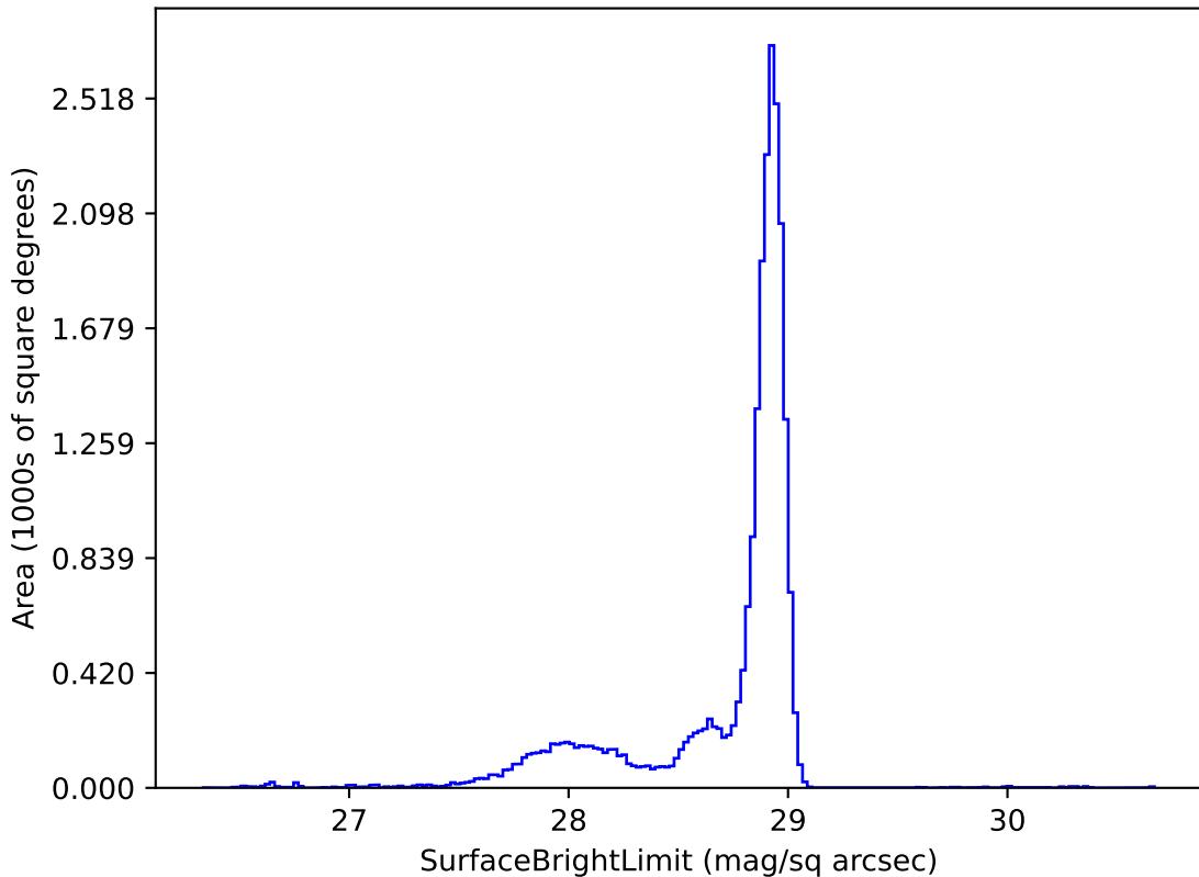
roll_pause_mjdp365_v3.4_10yrs u: SurfaceBrightLimit
