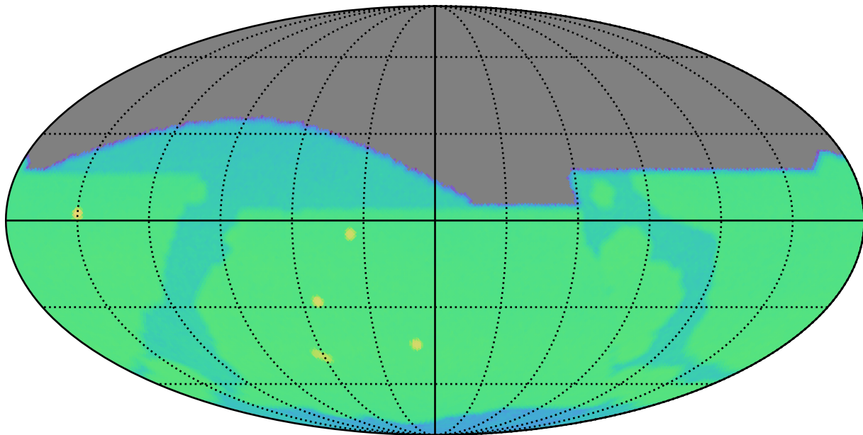
roll_pause_mjdp365_v3.4_10yrs r: SurfaceBrightLimit
