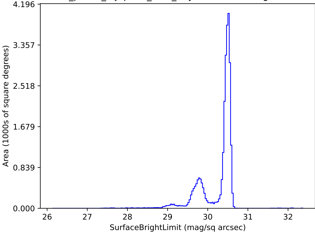
roll_pause_mjdp365_v3.4_10yrs r: SurfaceBrightLimit
