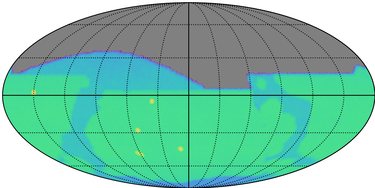
roll_pause_mjdp365_v3.4_10yrs i: SurfaceBrightLimit
