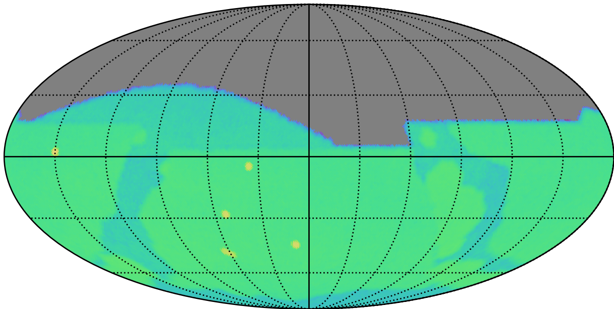
roll_pause_mjdp365_v3.4_10yrs g: SurfaceBrightLimit
