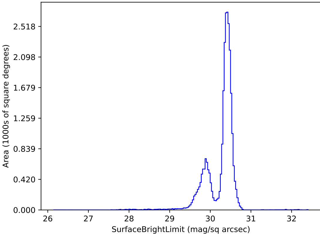
roll_pause_mjdp365_v3.4_10yrs g: SurfaceBrightLimit
