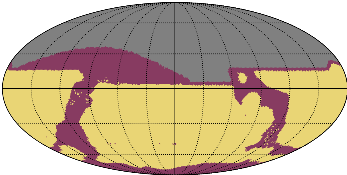
roll_pause_mjdp365_v3.4_10yrs : RapidRevisits
