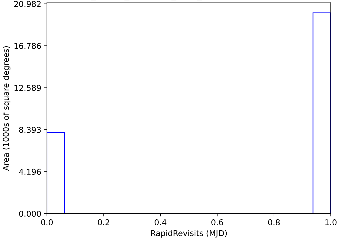
roll_pause_mjdp365_v3.4_10yrs : RapidRevisits
