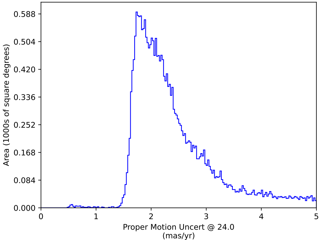
roll_pause_mjdp365_v3.4_10yrs : Proper Motion Uncert @ 24.0
