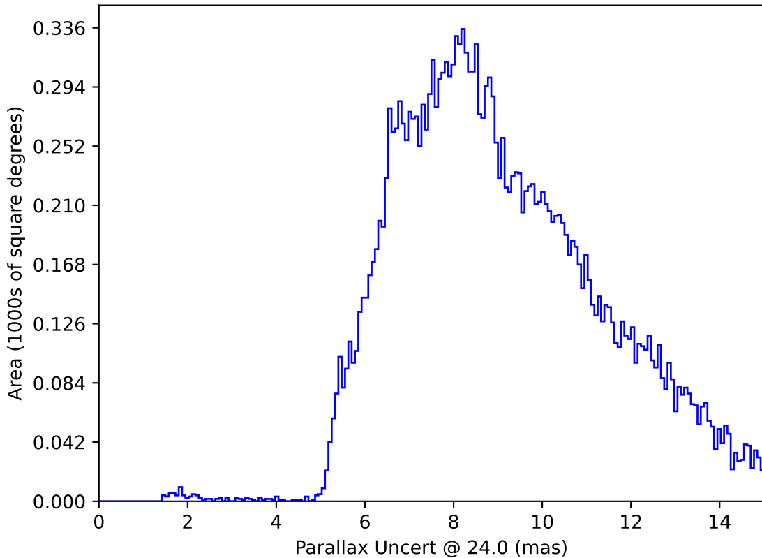
roll_pause_mjdp365_v3.4_10yrs : Parallax Uncert @ 24.0
