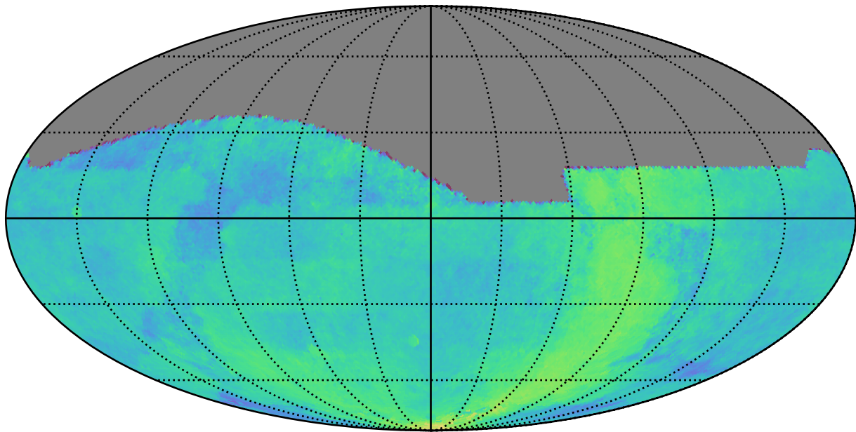
roll_pause_mjdp365_v3.4_10yrs : Parallax Coverage @ 24.0
