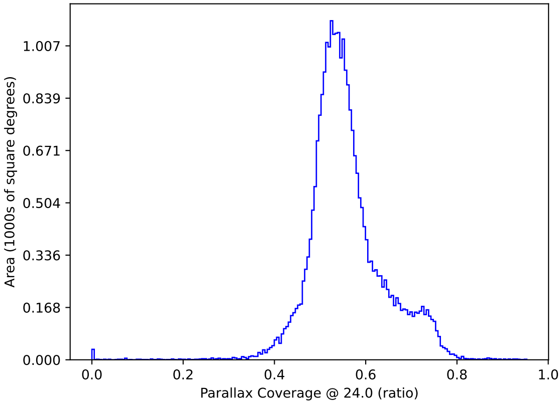
roll_pause_mjdp365_v3.4_10yrs : Parallax Coverage @ 24.0
