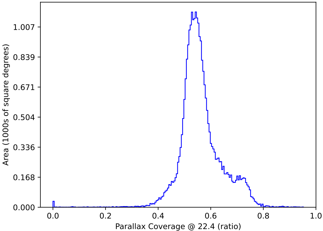
roll_pause_mjdp365_v3.4_10yrs : Parallax Coverage @ 22.4
