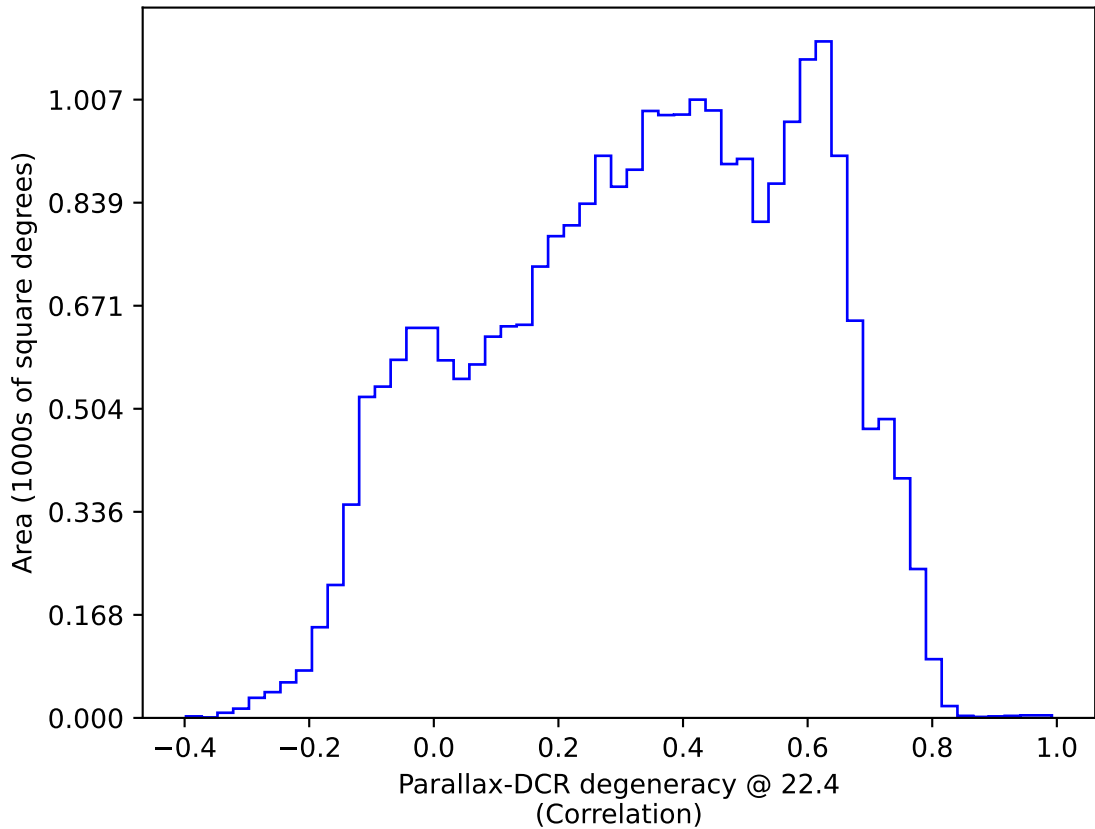
roll_pause_mjdp365_v3.4_10yrs : Parallax-DCR degeneracy @ 22.4
