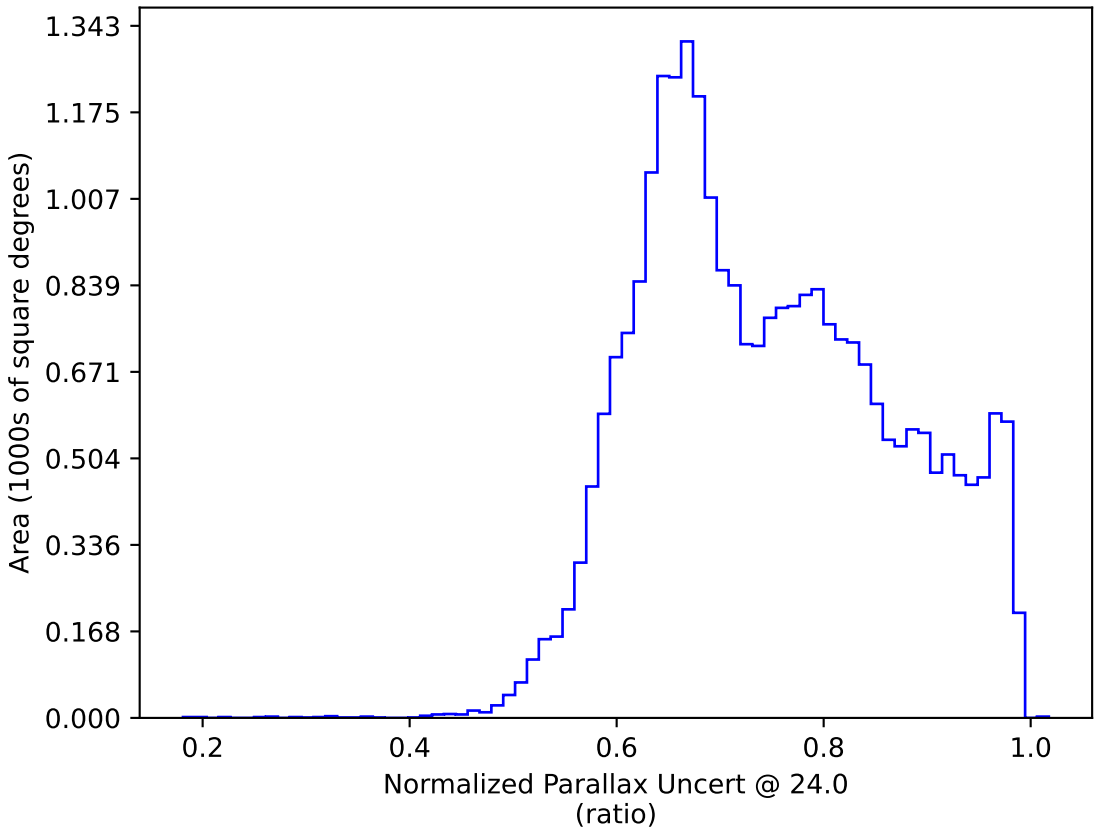
roll_pause_mjdp365_v3.4_10yrs : Normalized Parallax Uncert @ 24.0
