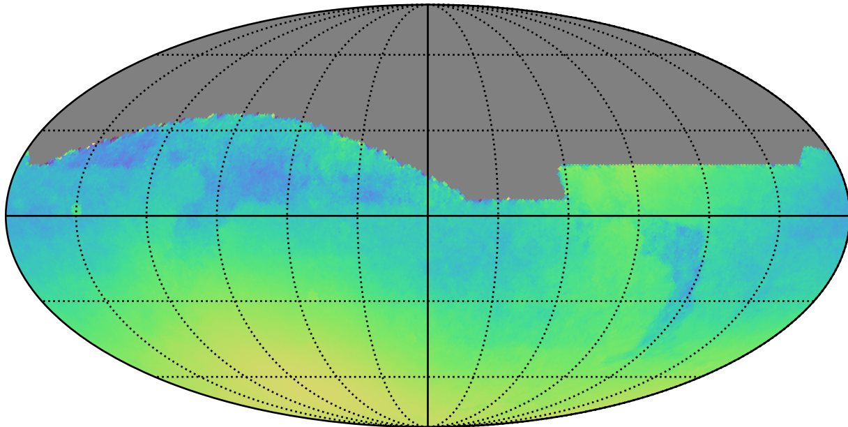
roll_pause_mjdp365_v3.4_10yrs : Normalized Parallax Uncert @ 22.4
