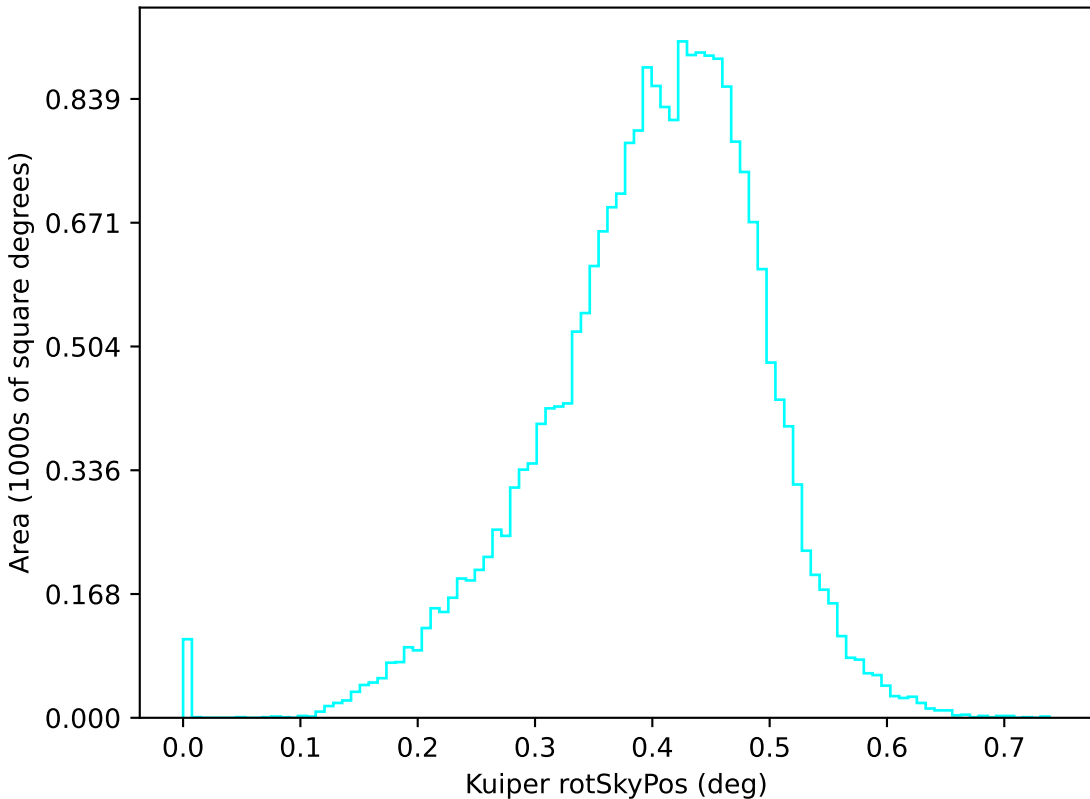
roll_pause_mjdp365_v3.4_10yrs u: Kuiper rotSkyPos
