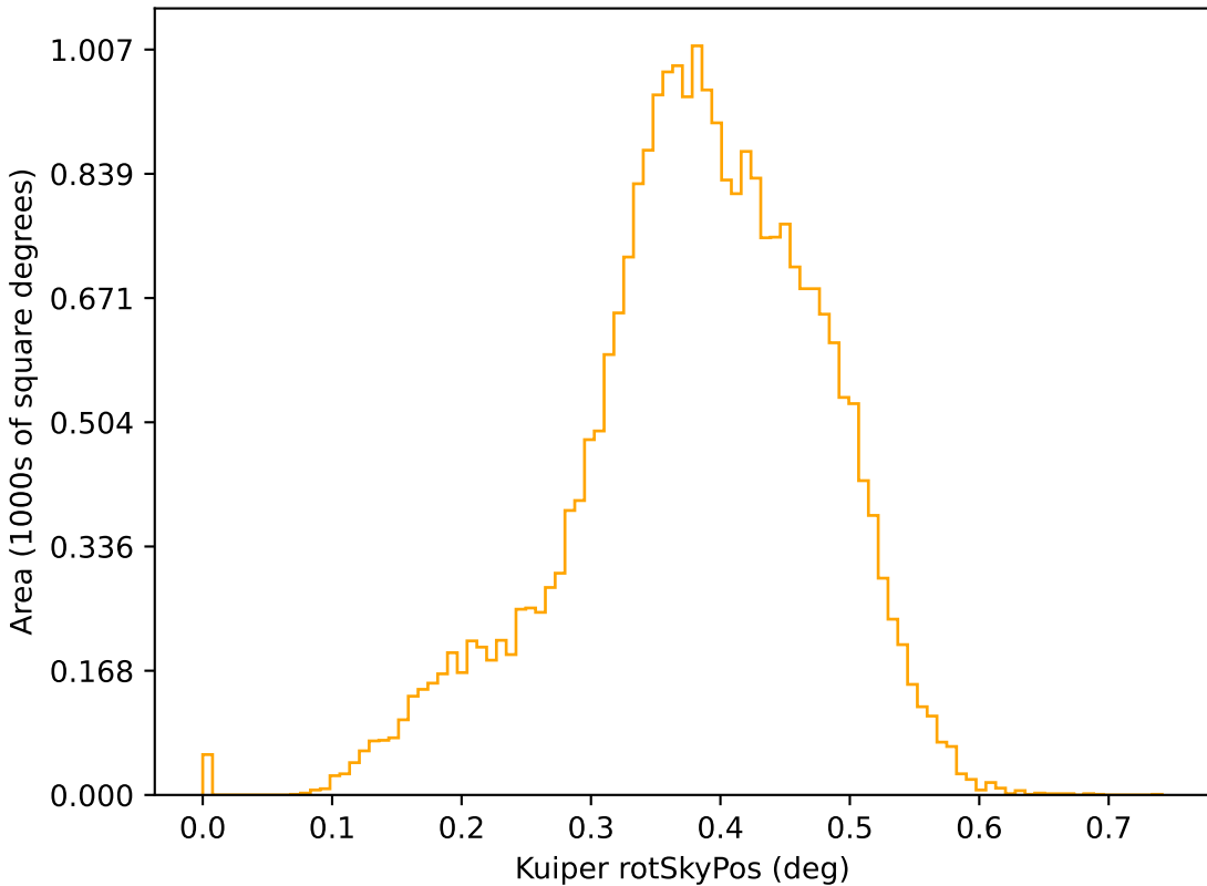
roll_pause_mjdp365_v3.4_10yrs r: Kuiper rotSkyPos
