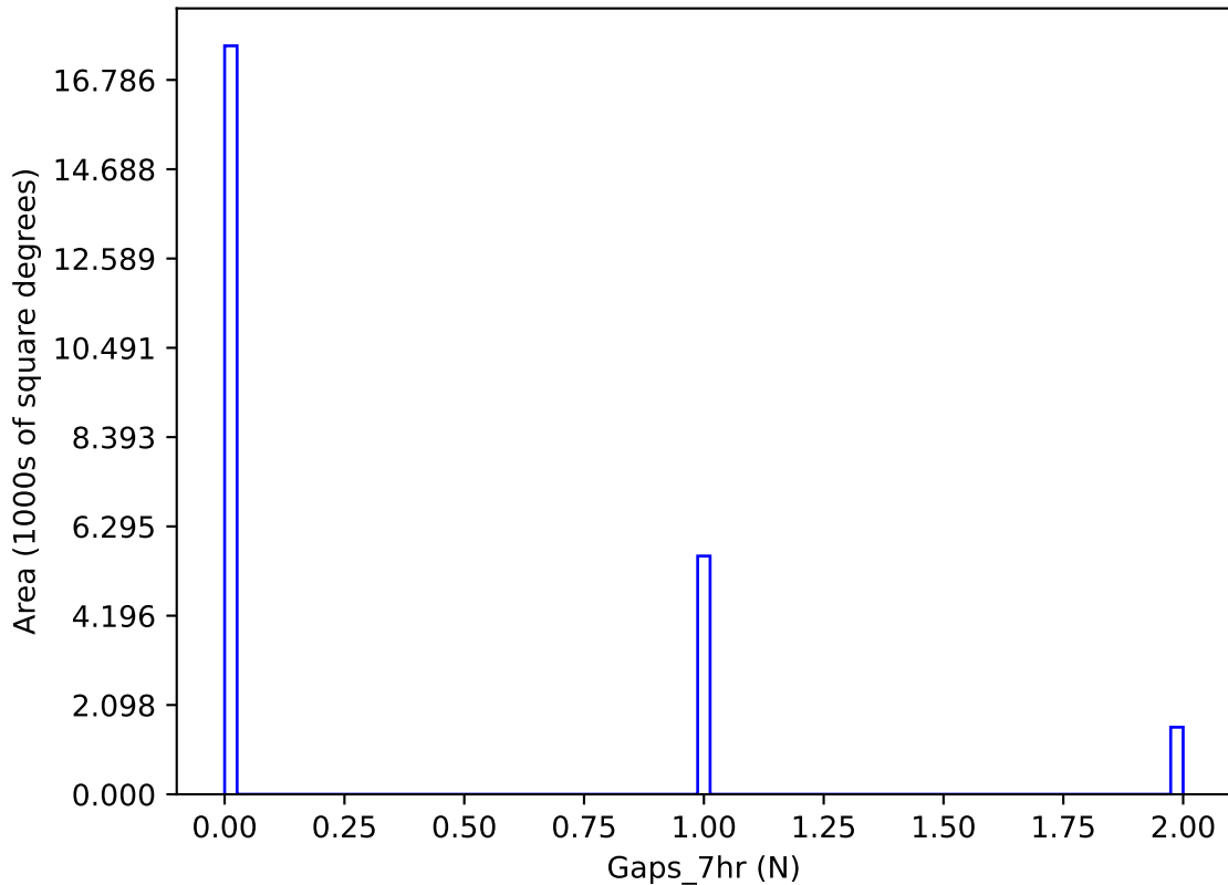
roll_pause_mjdp365_v3.4_10yrs y band: Gaps_7hr
