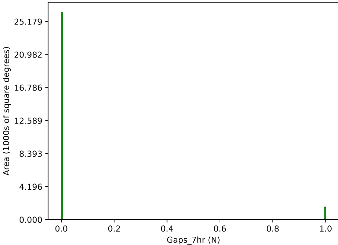
roll_pause_mjdp365_v3.4_10yrs g band: Gaps_7hr
