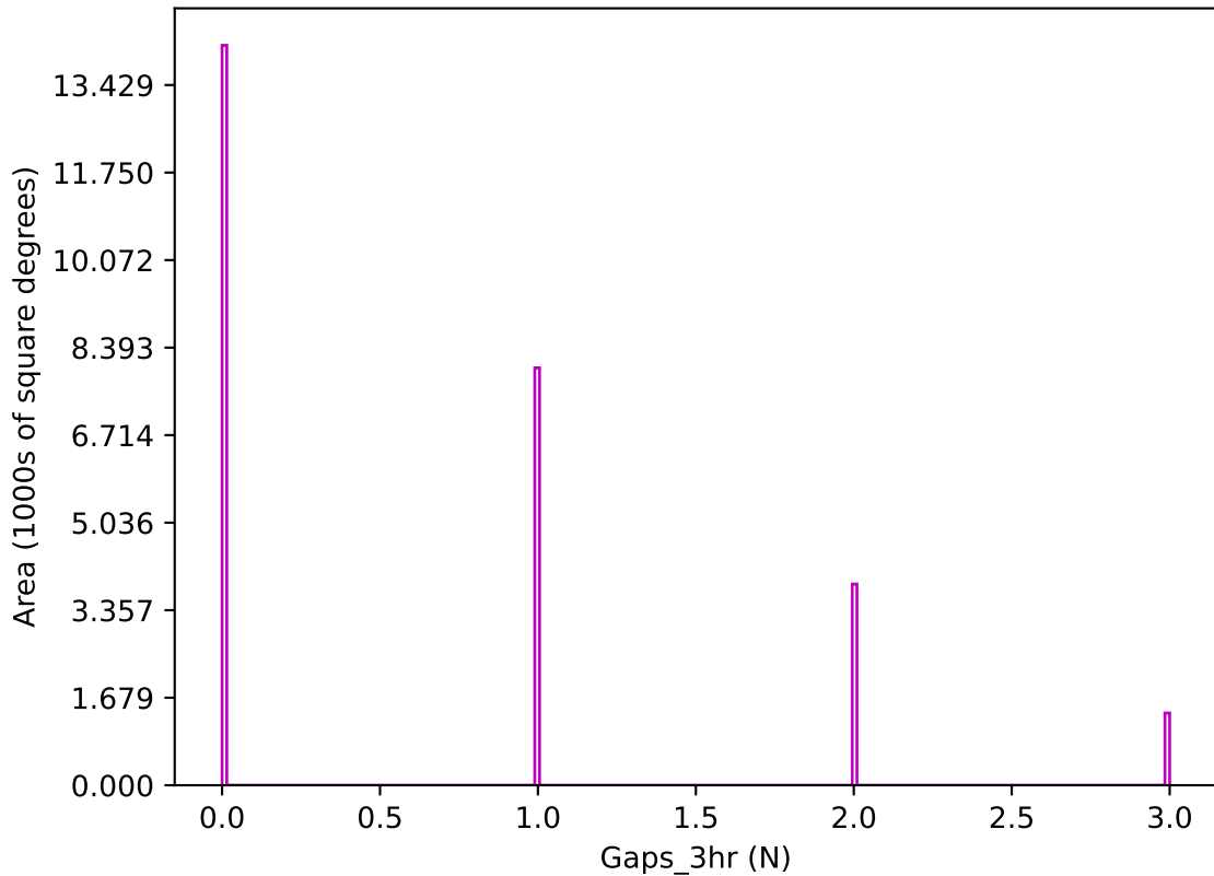
roll_pause_mjdp365_v3.4_10yrs z band: Gaps_3hr
