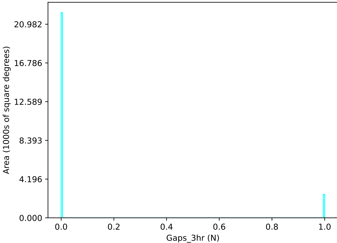
roll_pause_mjdp365_v3.4_10yrs u band: Gaps_3hr
