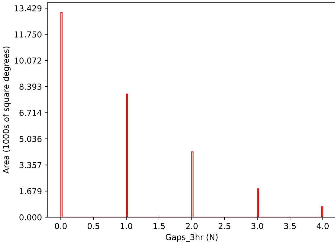
roll_pause_mjdp365_v3.4_10yrs i band: Gaps_3hr
