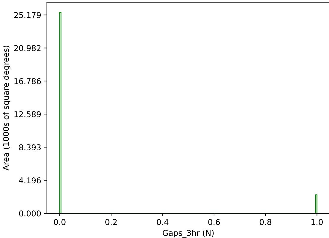
roll_pause_mjdp365_v3.4_10yrs g band: Gaps_3hr
