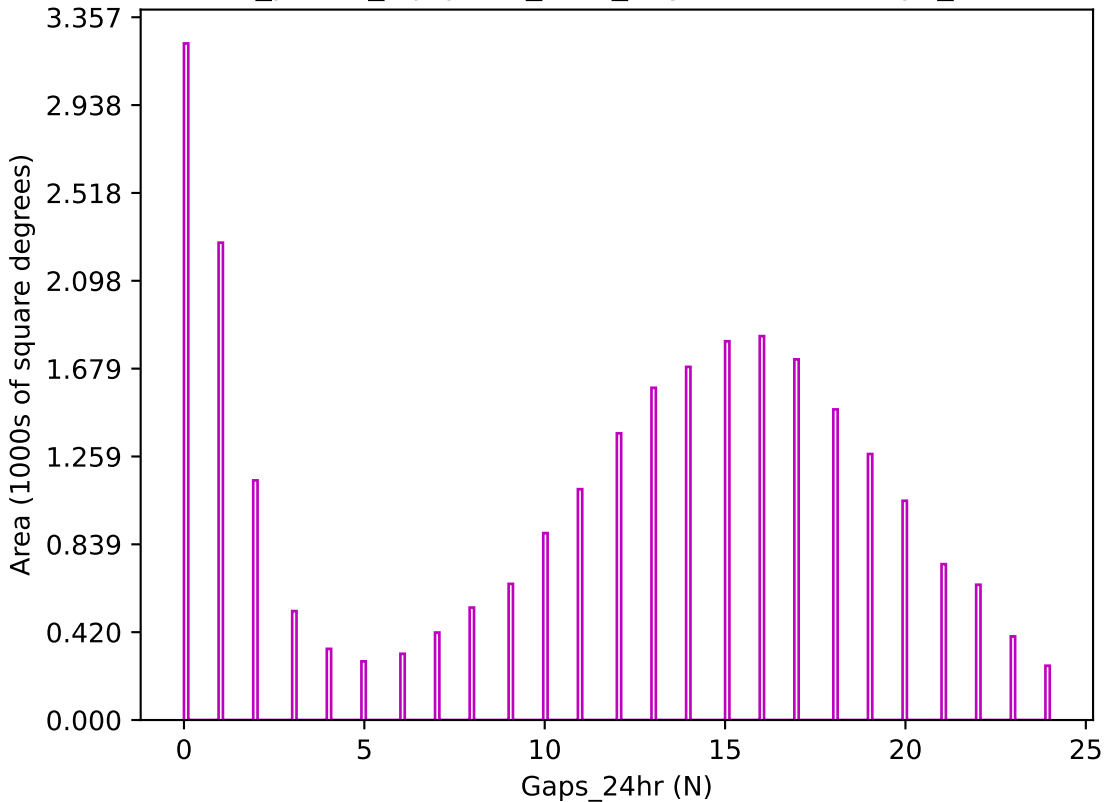
roll_pause_mjdp365_v3.4_10yrs z band: Gaps_24hr
