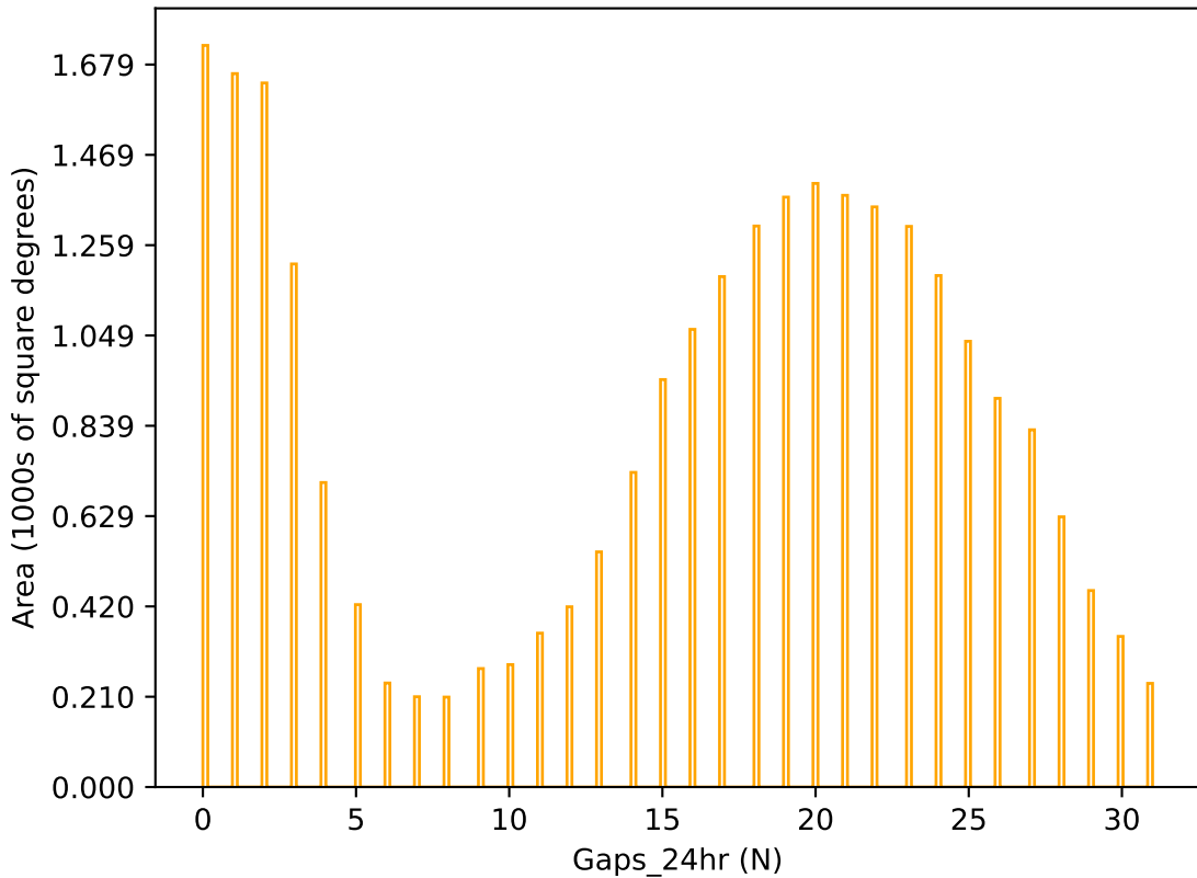
roll_pause_mjdp365_v3.4_10yrs r band: Gaps_24hr
