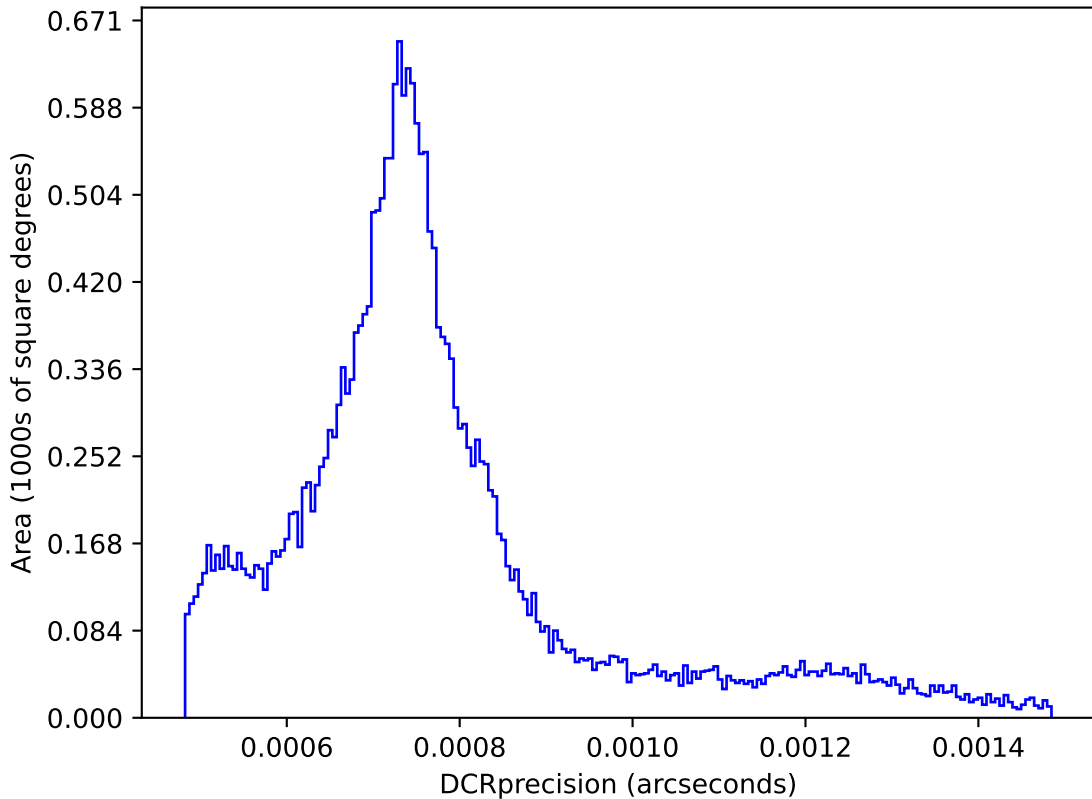
roll_pause_mjdp365_v3.4_10yrs : DCRprecision
