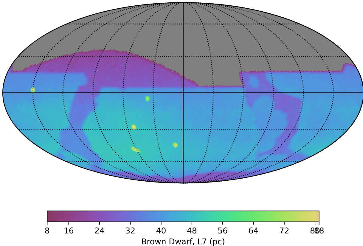
roll_pause_mjdp365_v3.4_10yrs : Brown Dwarf, L7
