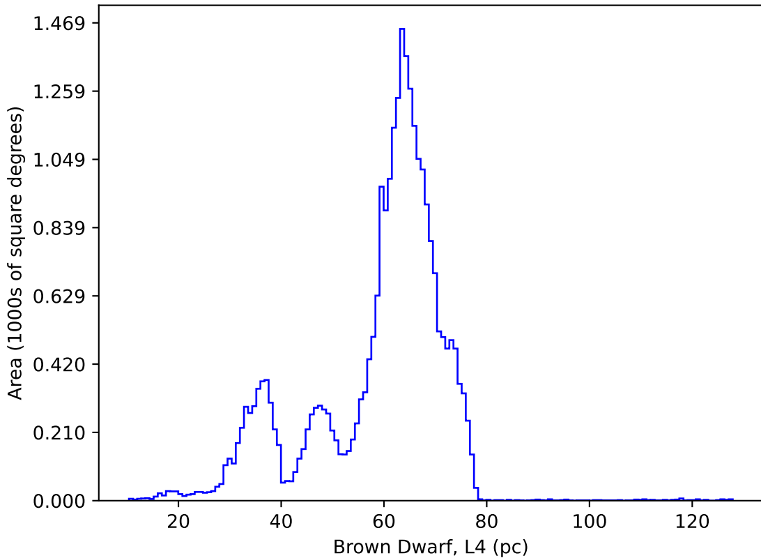
roll_pause_mjdp365_v3.4_10yrs : Brown Dwarf, L4
