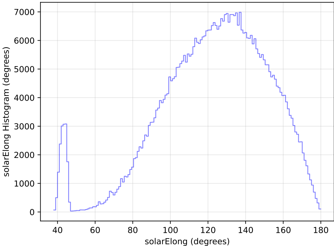
roll_pause_mjdp365_v3.4_10yrs WFD r band: solarElong Histogram
