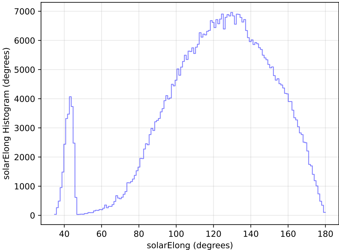
roll_pause_mjdp365_v3.4_10yrs WFD i band: solarElong Histogram
