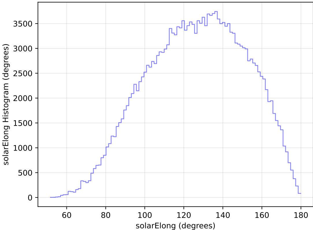
roll_pause_mjdp365_v3.4_10yrs WFD g band: solarElong Histogram
