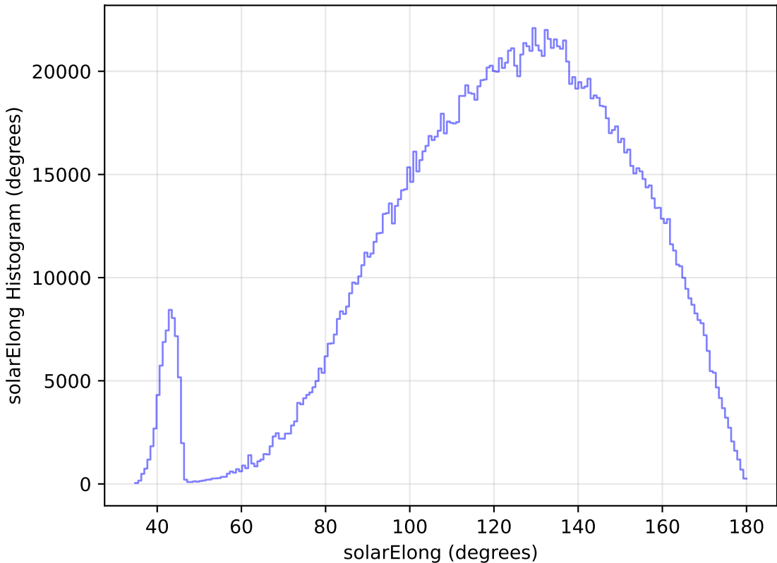
roll_pause_mjdp365_v3.4_10yrs WFD all bands: solarElong Histogram
