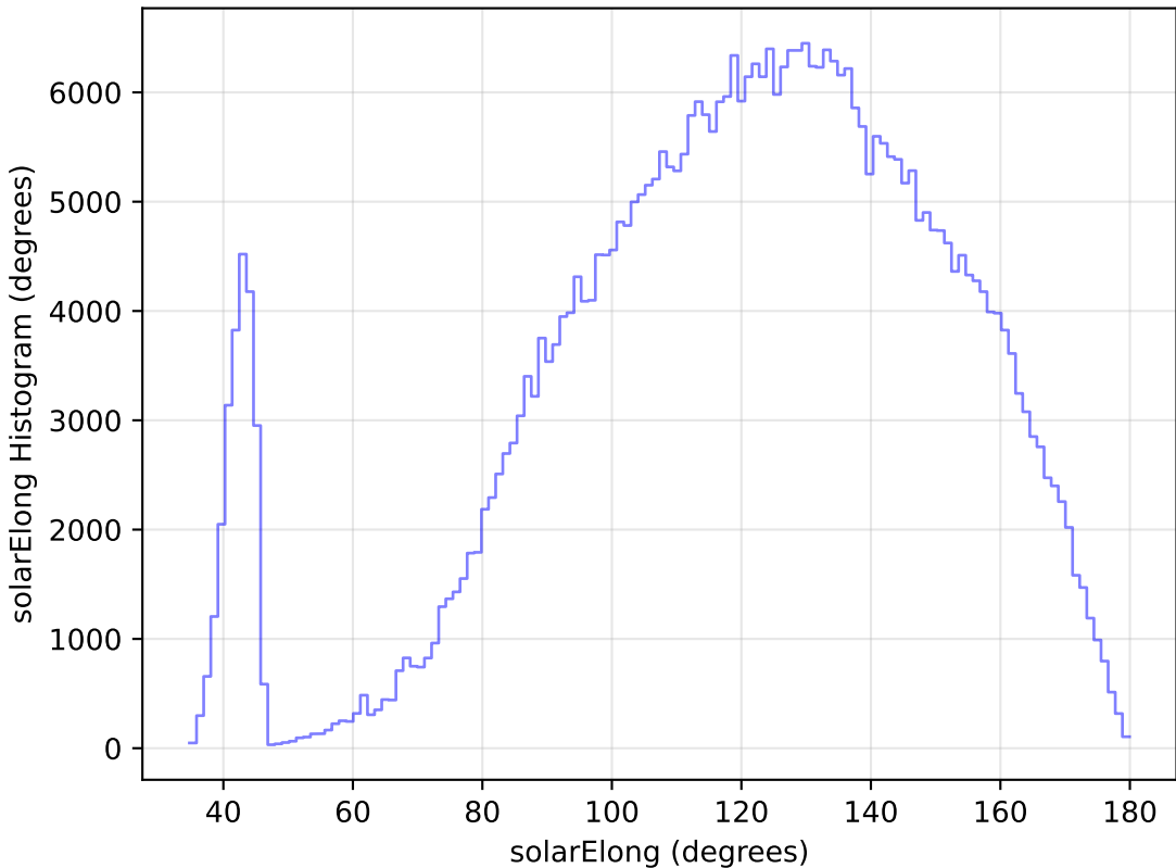
roll_pause_mjdp365_v3.4_10yrs All sky z band: solarElong Histogram
