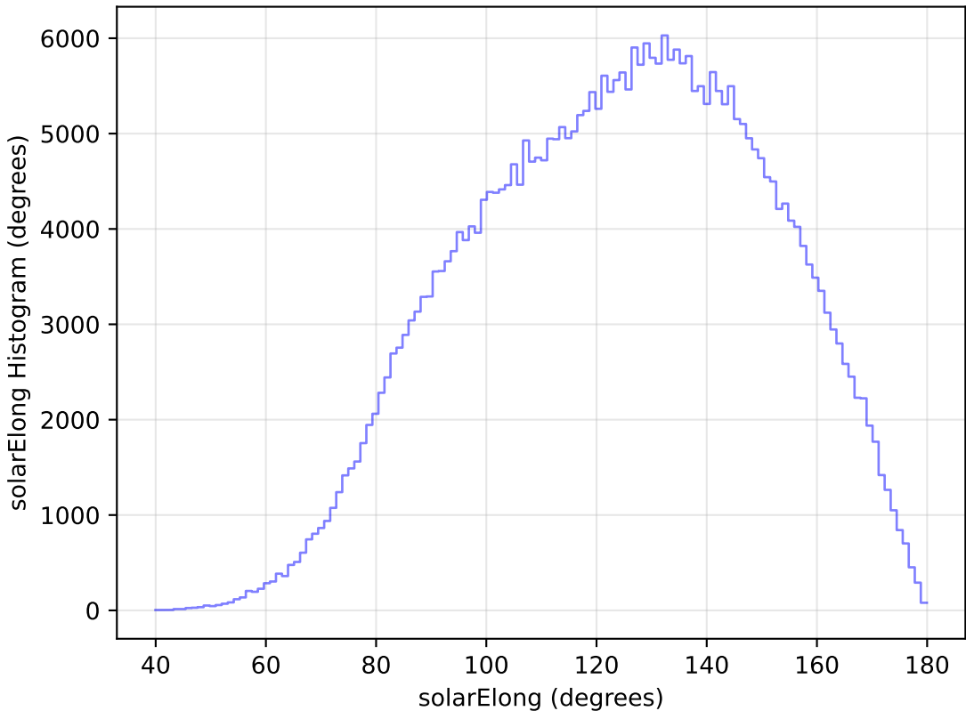
roll_pause_mjdp365_v3.4_10yrs All sky y band: solarElong Histogram
