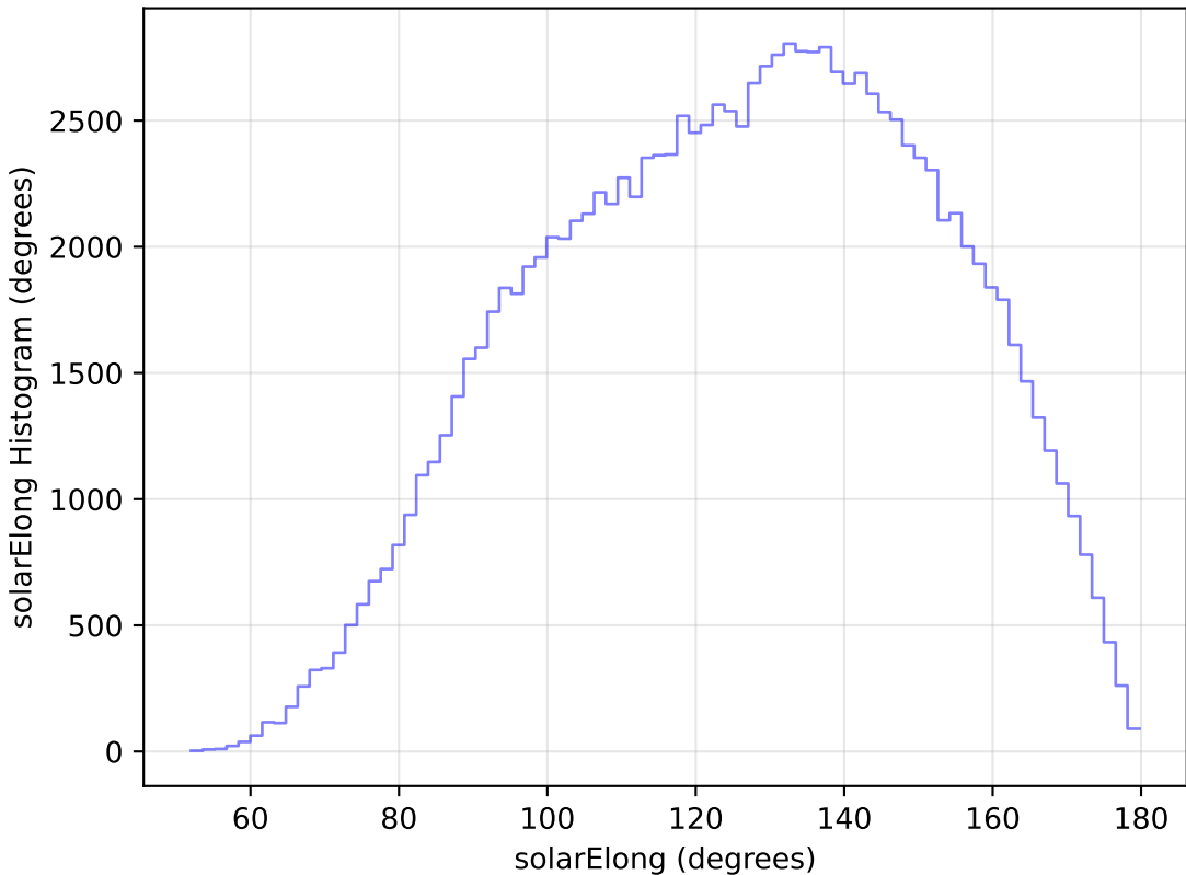
roll_pause_mjdp365_v3.4_10yrs All sky u band: solarElong Histogram
