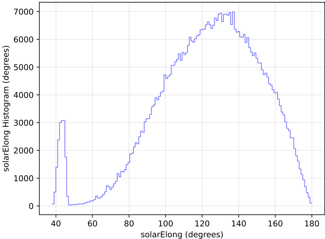
roll_pause_mjdp365_v3.4_10yrs All sky r band: solarElong Histogram
