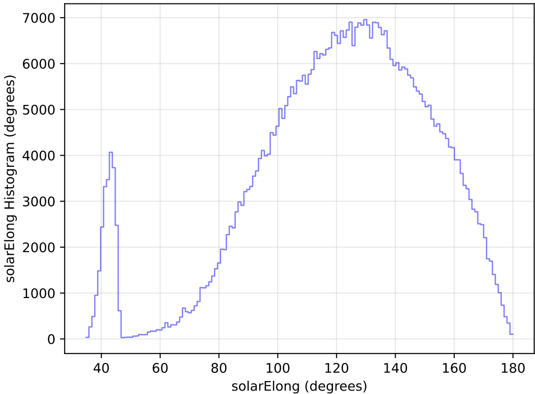
roll_pause_mjdp365_v3.4_10yrs All sky i band: solarElong Histogram
