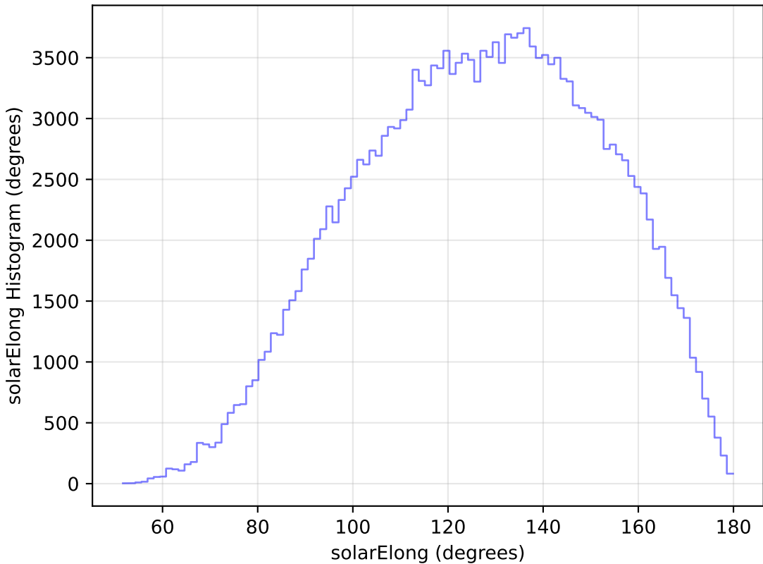
roll_pause_mjdp365_v3.4_10yrs All sky g band: solarElong Histogram
