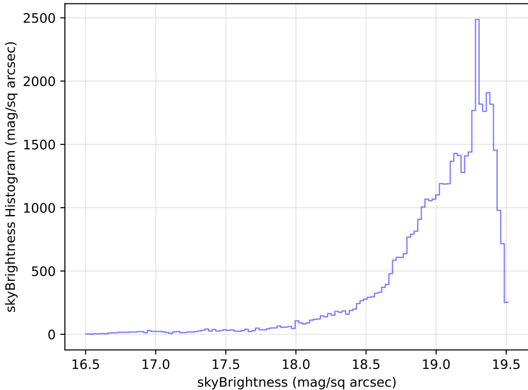
roll_pause_mjdp365_v3.4_10yrs Yr 1 z band: skyBrightness Histogram
