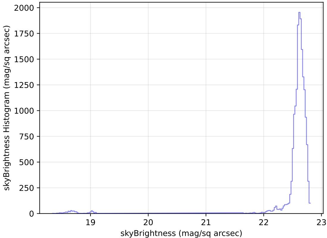
roll_pause_mjdp365_v3.4_10yrs Yr 1 u band: skyBrightness Histogram
