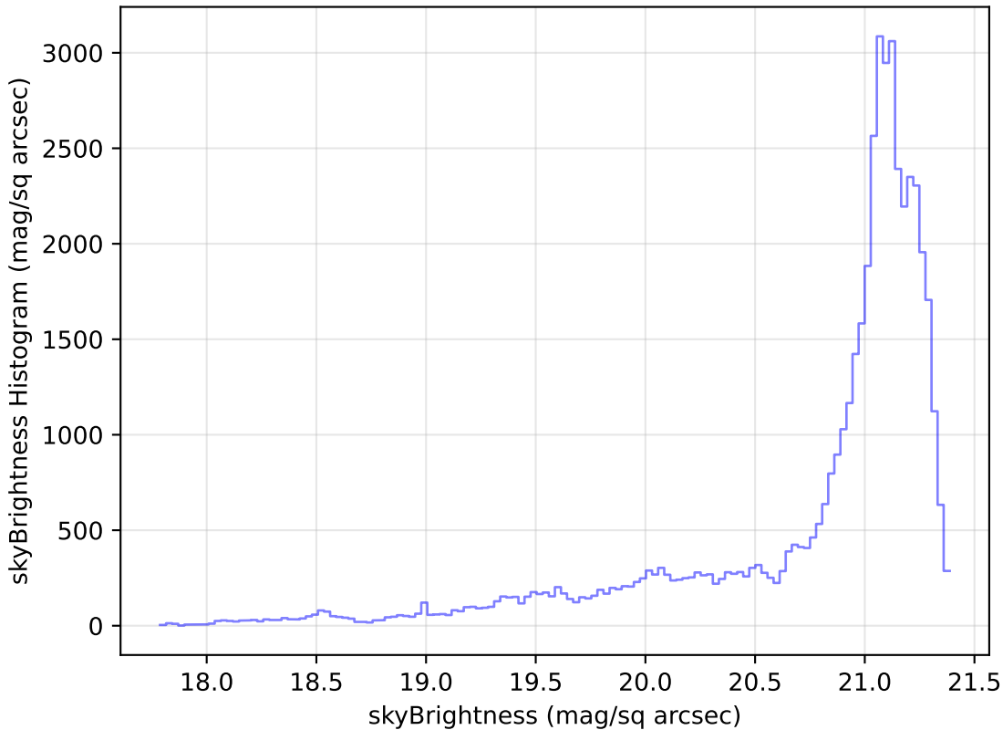
roll_pause_mjdp365_v3.4_10yrs Yr 1 r band: skyBrightness Histogram
