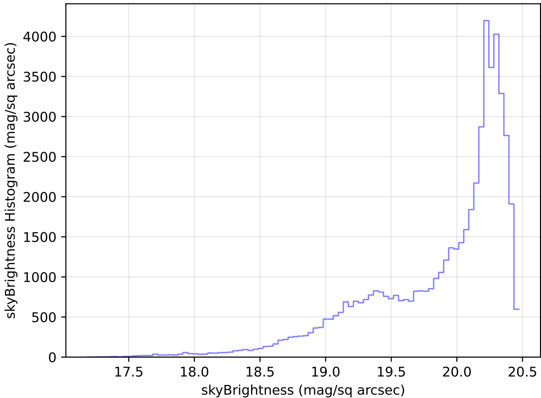
roll_pause_mjdp365_v3.4_10yrs Yr 1 i band: skyBrightness Histogram
