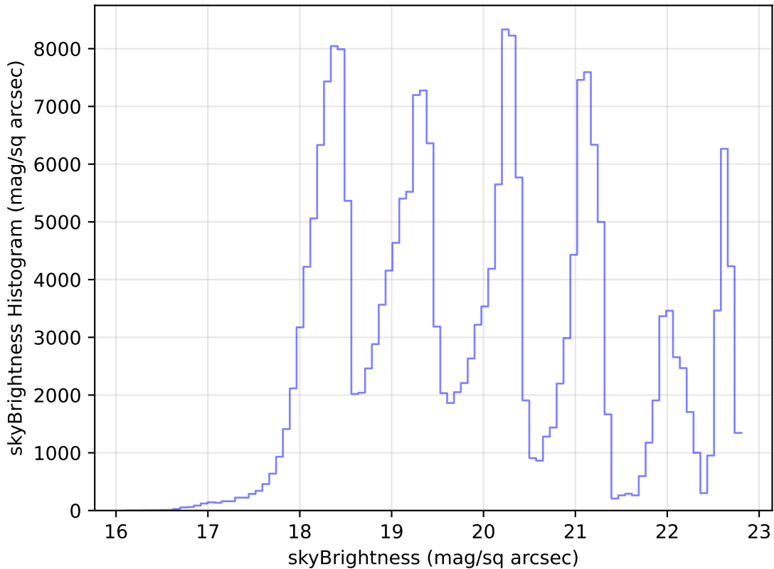
roll_pause_mjdp365_v3.4_10yrs Yr 1 all bands: skyBrightness Histogram
